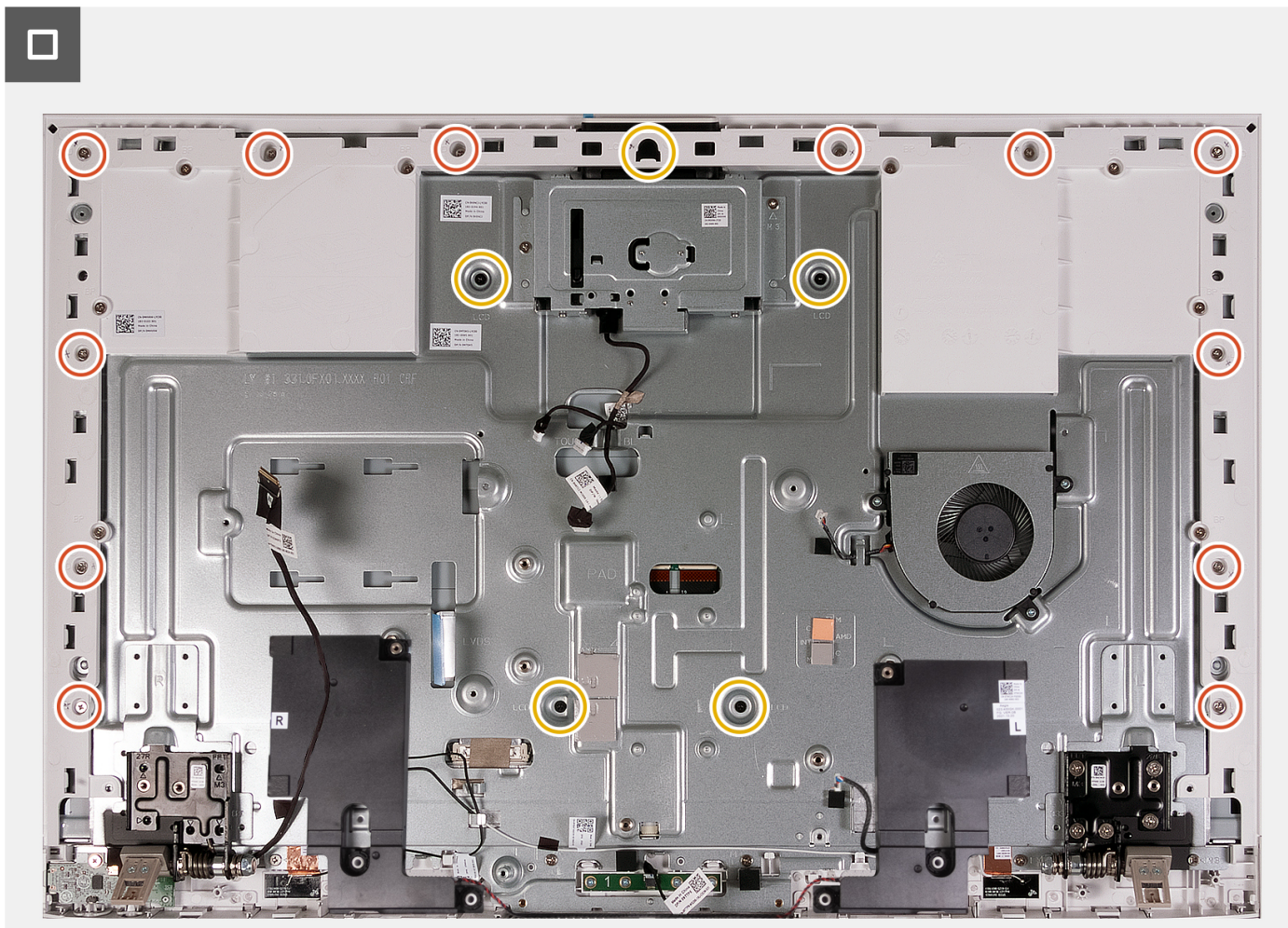
Figure 63. Replacing the screws
