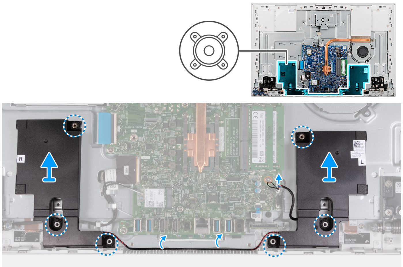
Figure 38. Removing the speakers
