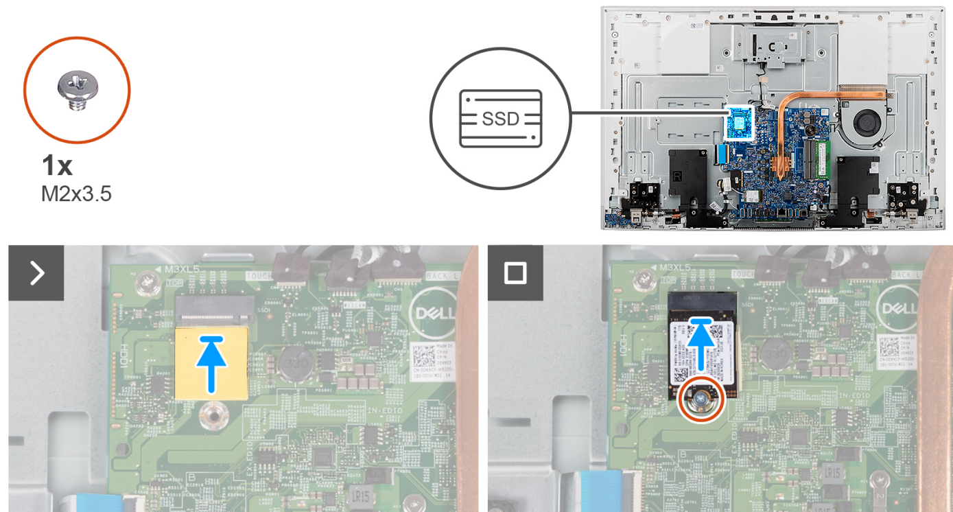
Figure 29. Installing the M.2 2230 solid-state drive
