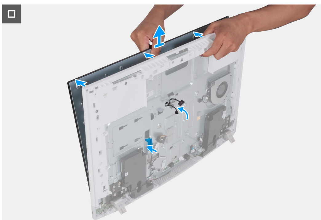
Figure 61. Removing the display panel
