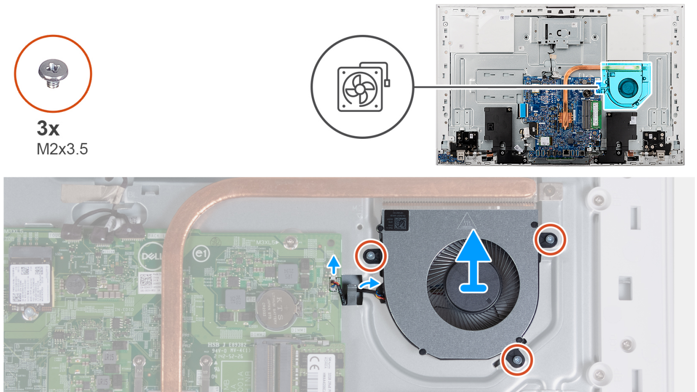
Figure 36. Removing the fan
