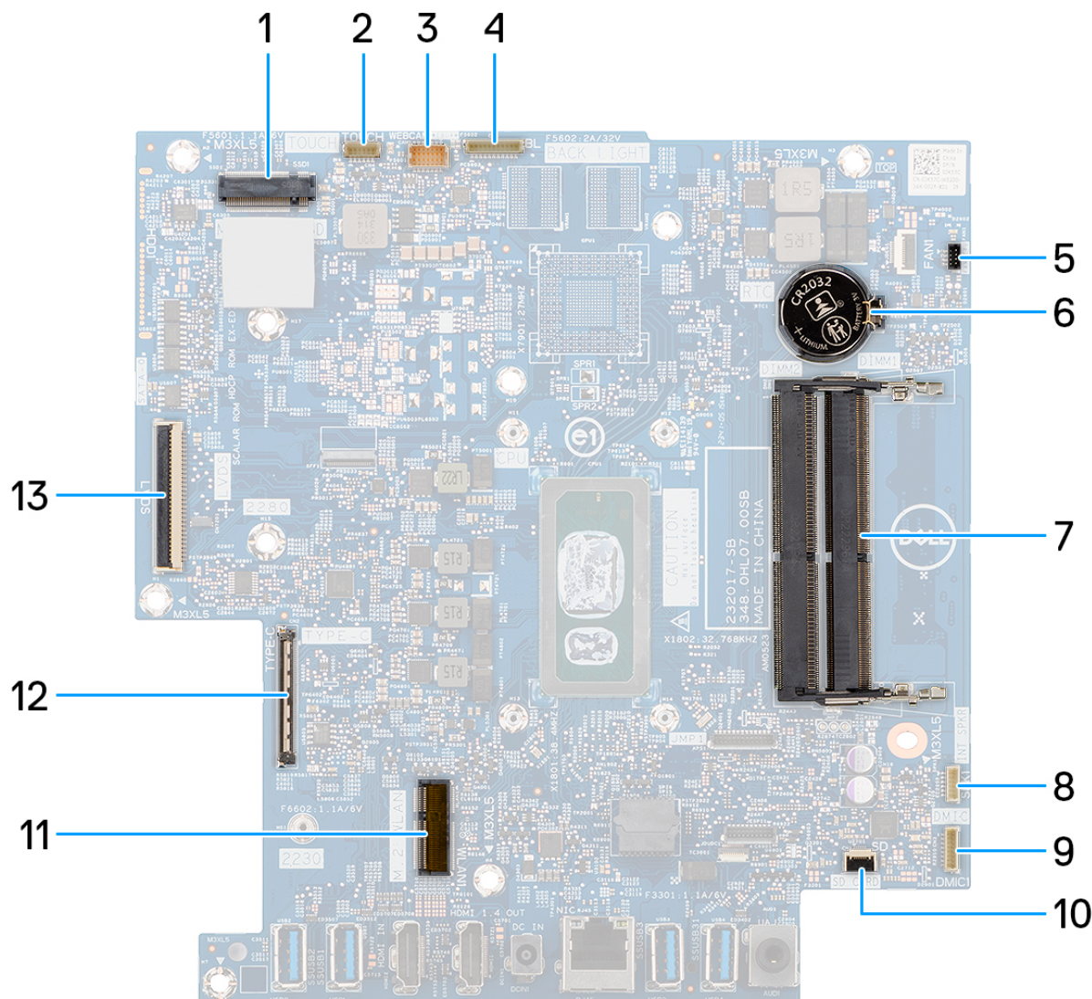
Figure 53. System-board connectors
