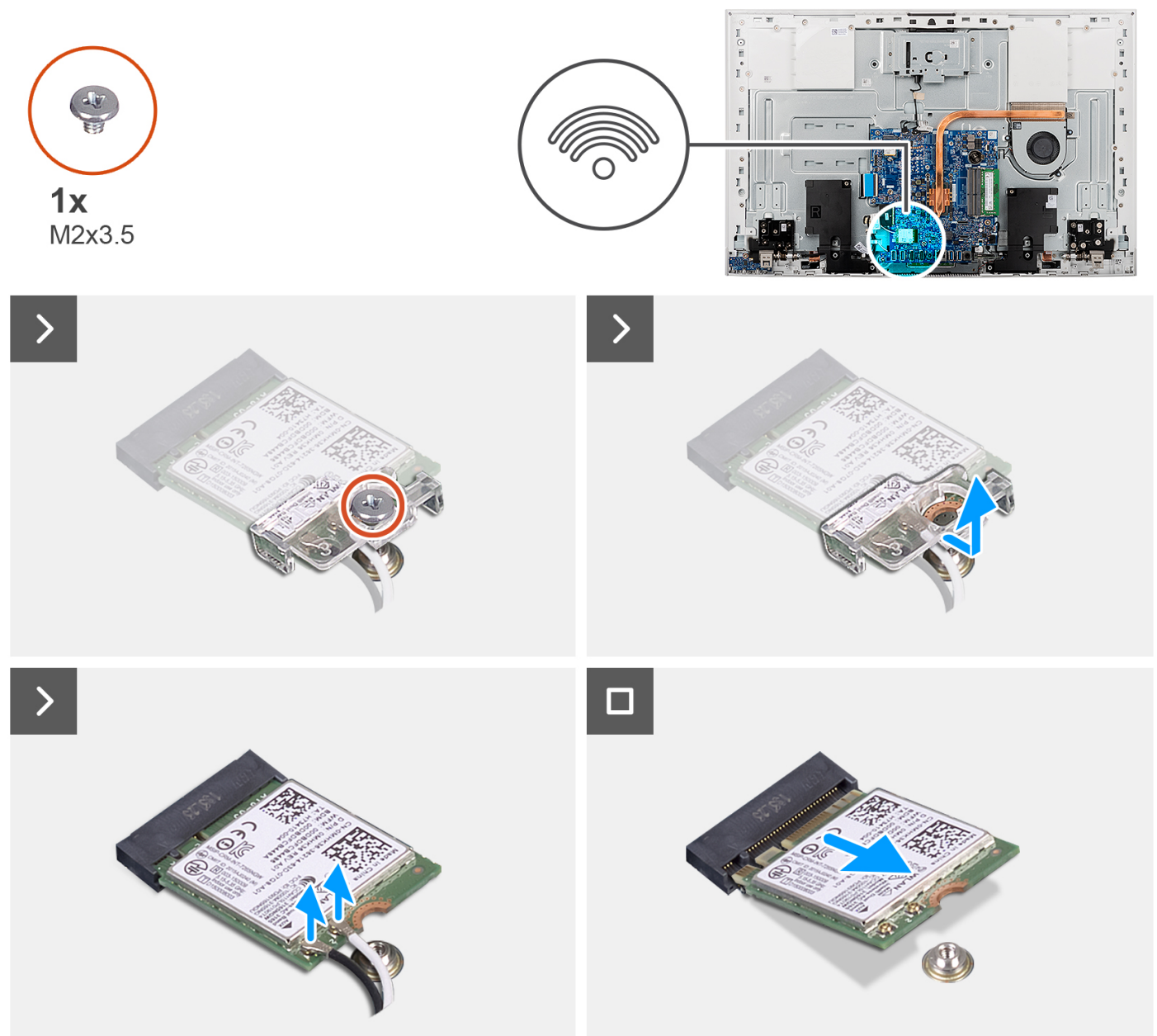
Figure 32. Removing the wireless card
