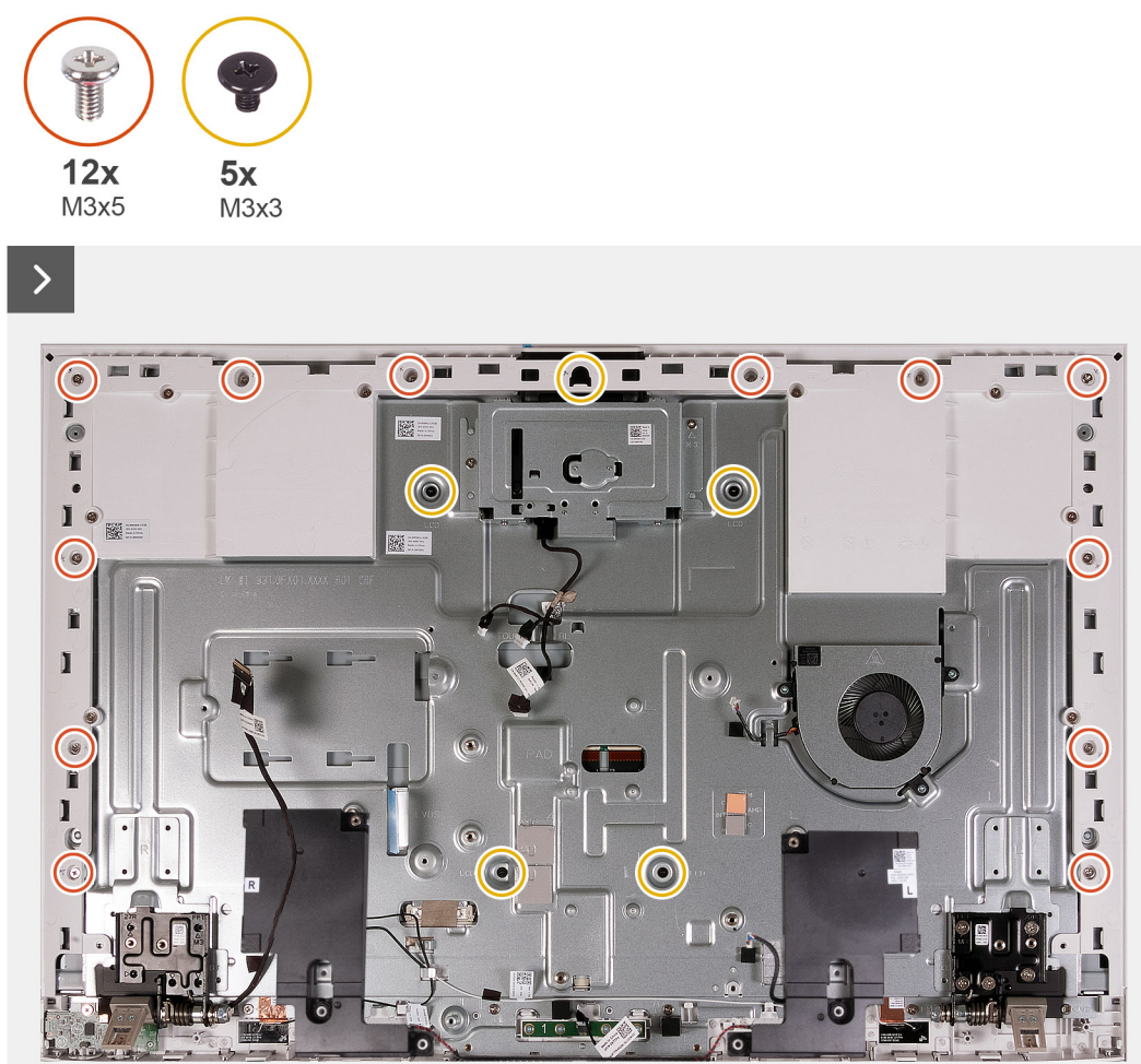
Figure 60. Removing the screws
