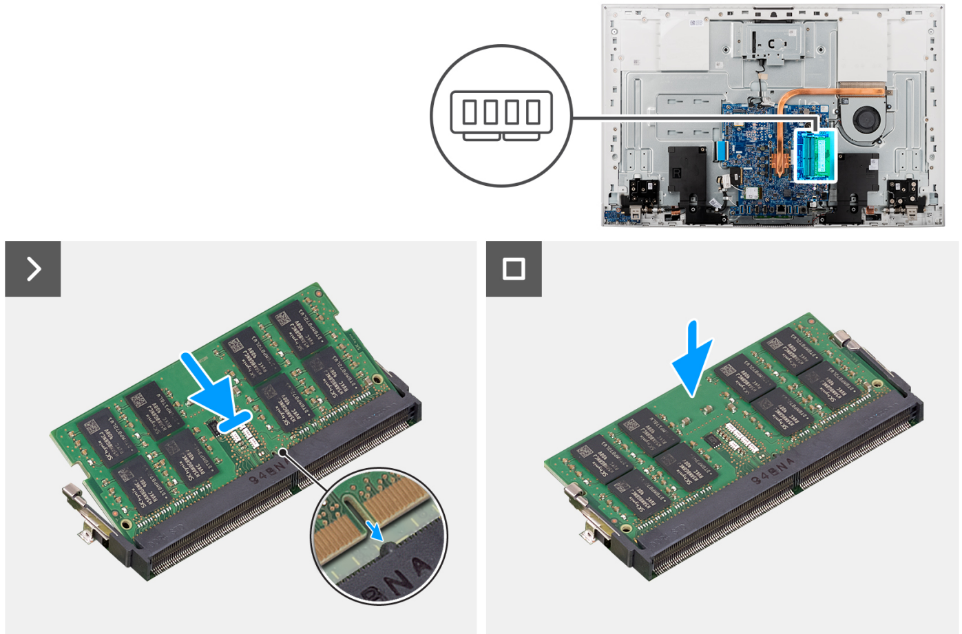
Figure 31. Installing the memory module
