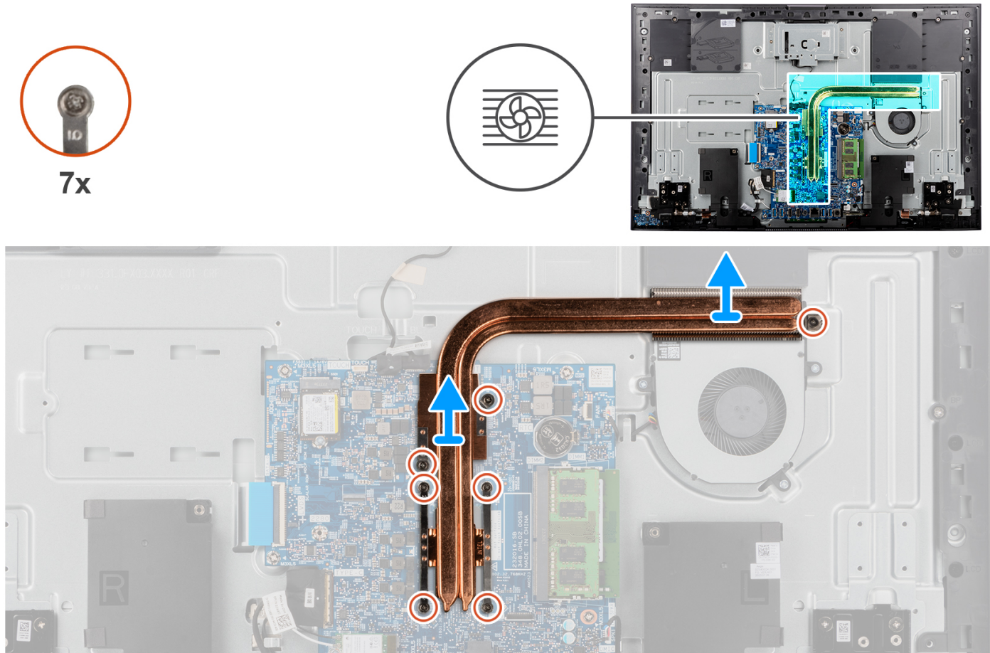
Figure 44. Removing the heat sink- discrete
