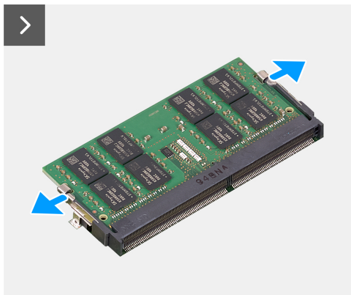
Figure 30. Removing the memory module
