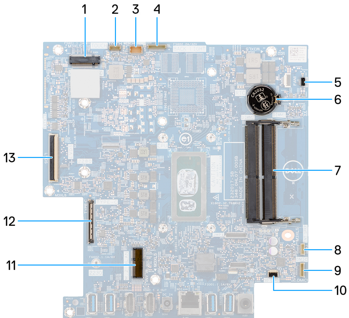
Figure 50. System-board connectors
