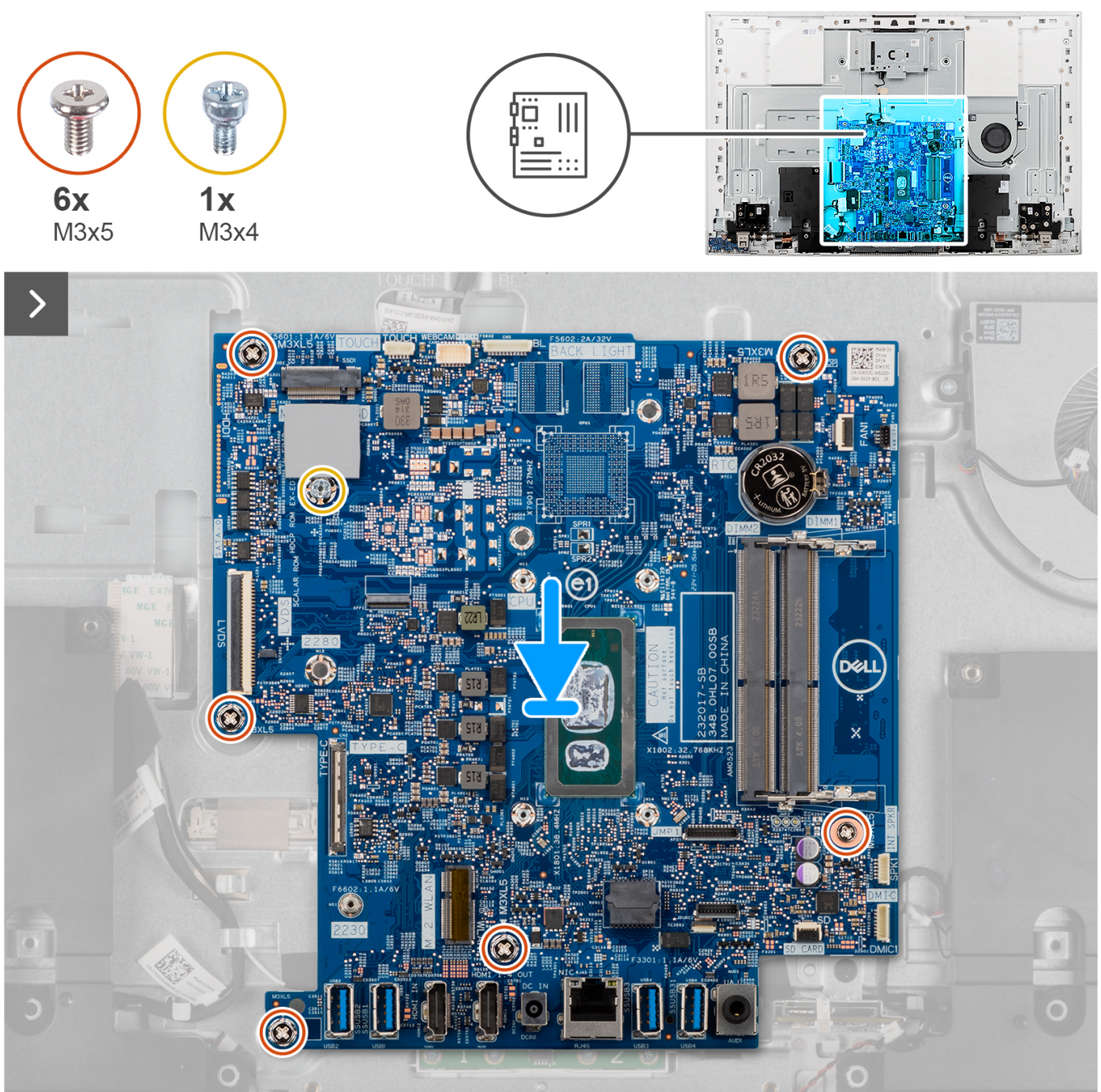
Figure 54. Placing the system board in the chassis
